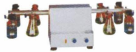
Shaking Machine (Wrist Action)
